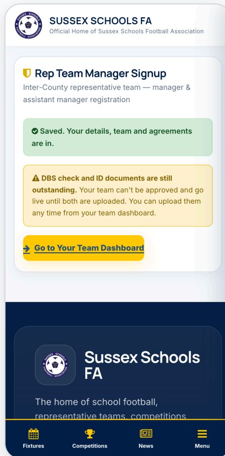
Confirmation screen
